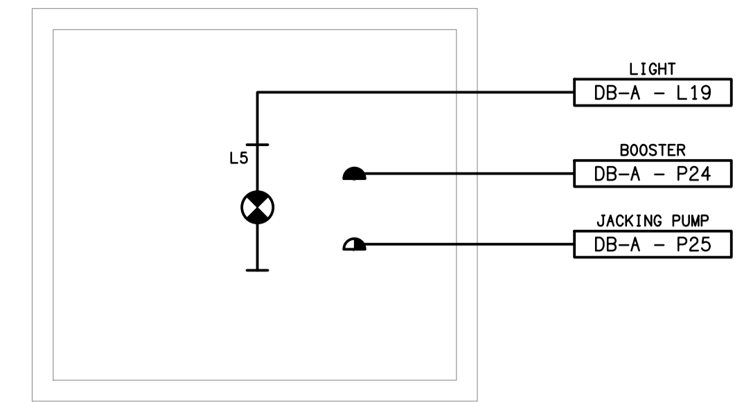
DETAIL A BOOSTER CABINET PLAN SCALE 1:50
